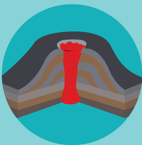
LAVA DOME VOLCANO
