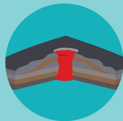
SHIELD VOLCANO
